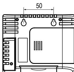
Dimensions for wall mounting
