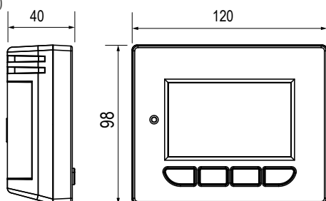
Dimensions for wall mounting
