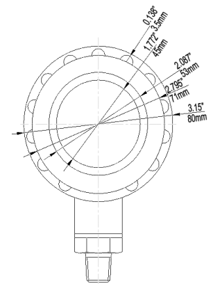
DPG SERIES with rubber cover
