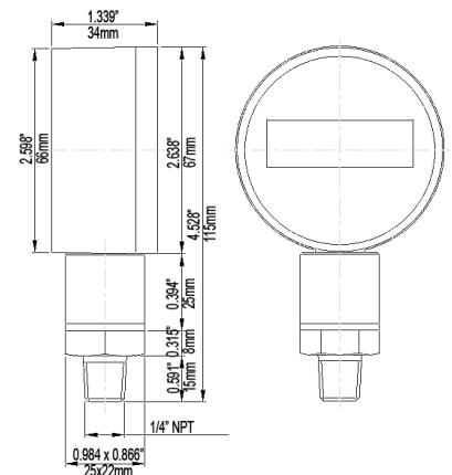
DPG SERIES without rubber cover
